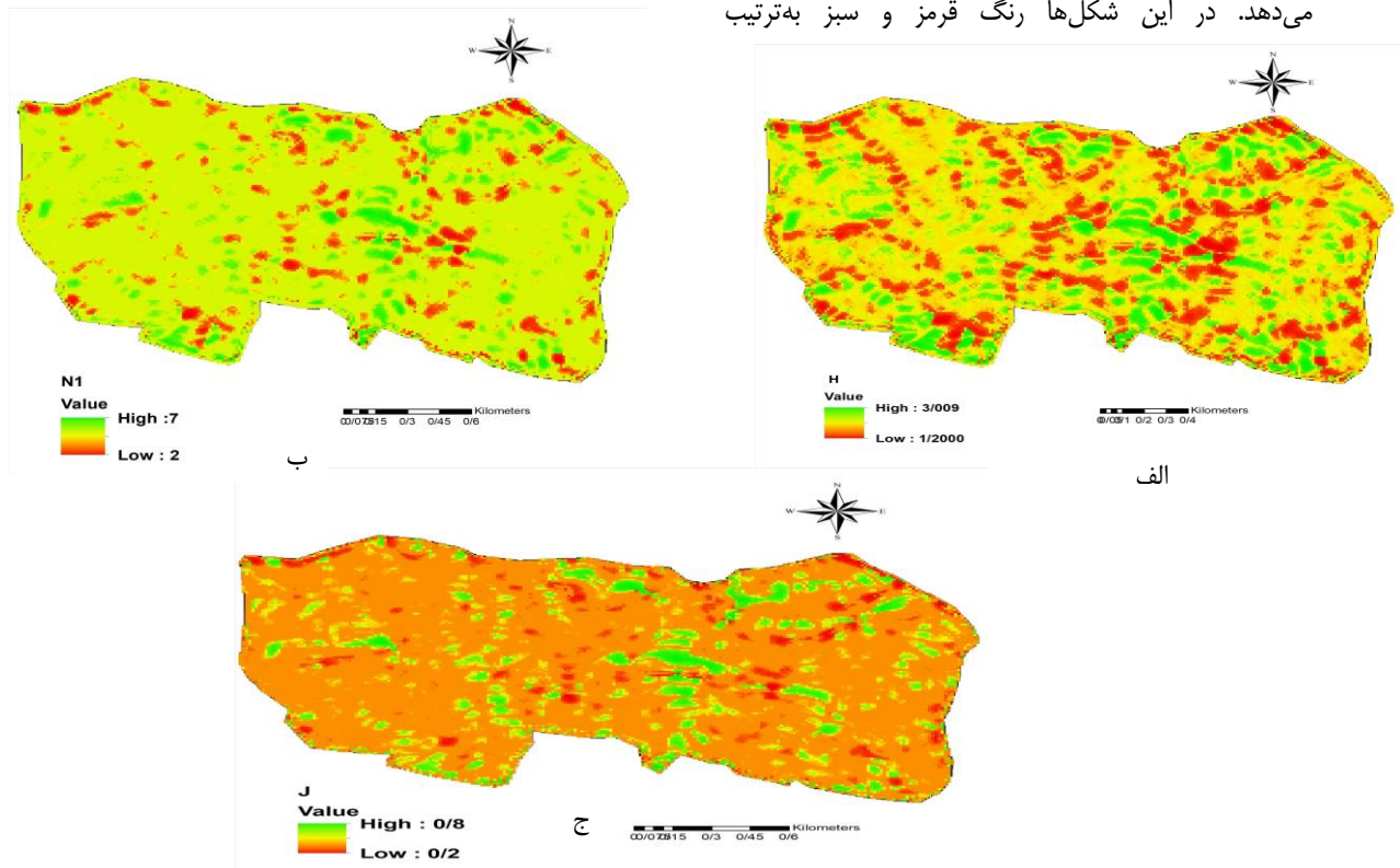
Figure 3. prepared Map using Geographically Weighted Regression model for diversity indices Shannon-wiener H (a), Hill N1 (b) and J Pielou (c)
