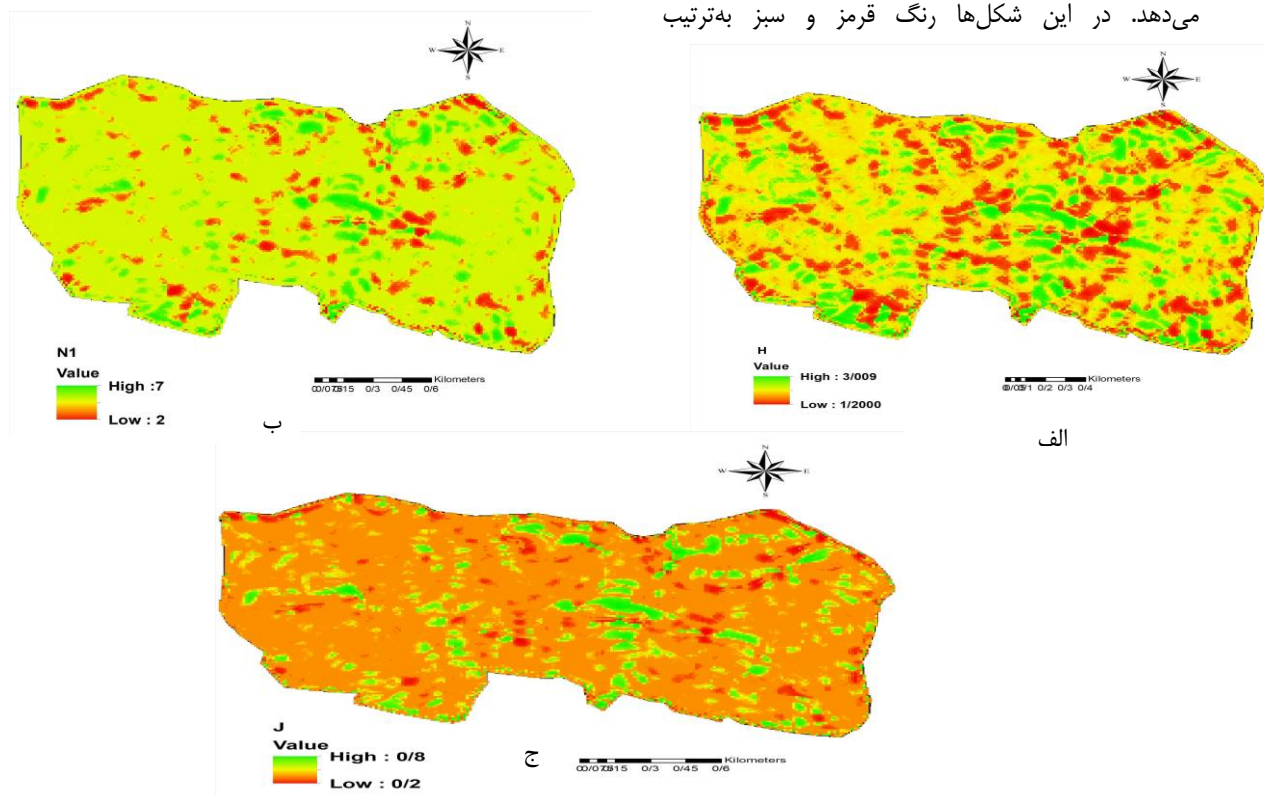
Figure 3. prepared Map using Geographically Weighted Regression model for diversity indices Shannon-wiener H (a), Hill N1 (b) and J Pillo (c)
